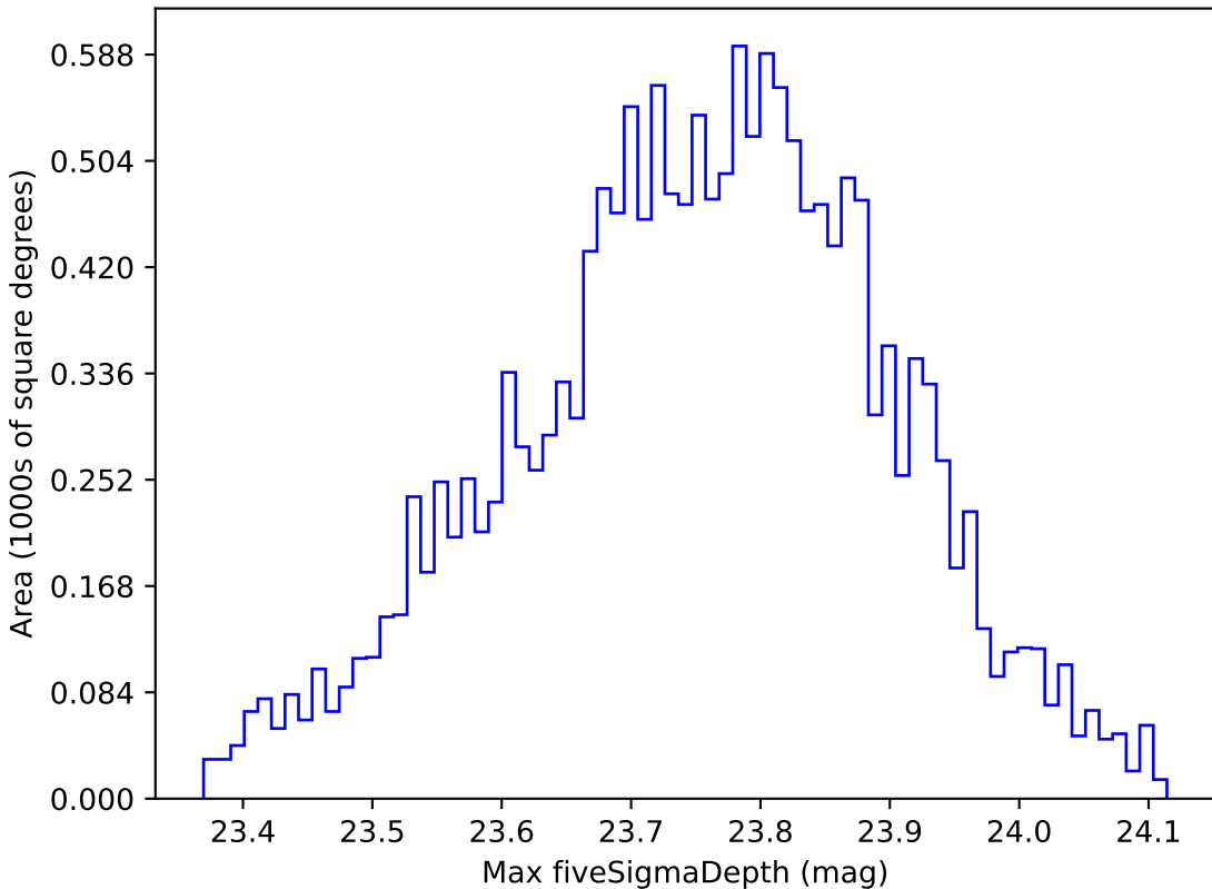
too_10_4v3.4_10yrs WFD u band: Max fiveSigmaDepth
