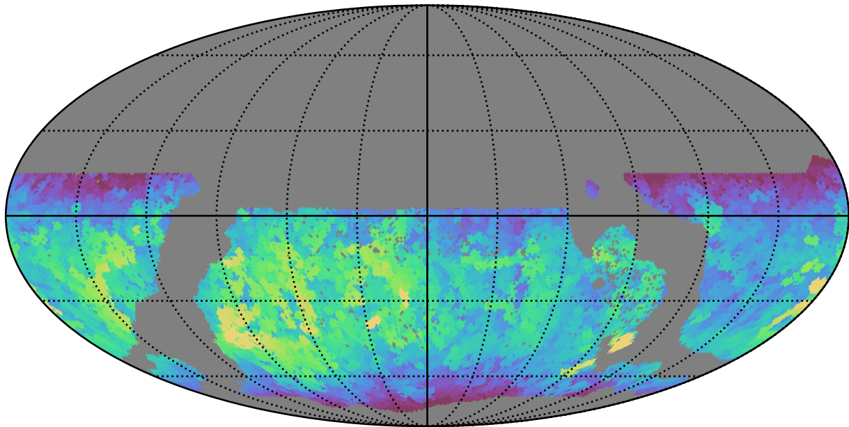
too_10_4v3.4_10yrs WFD i band: Max fiveSigmaDepth
