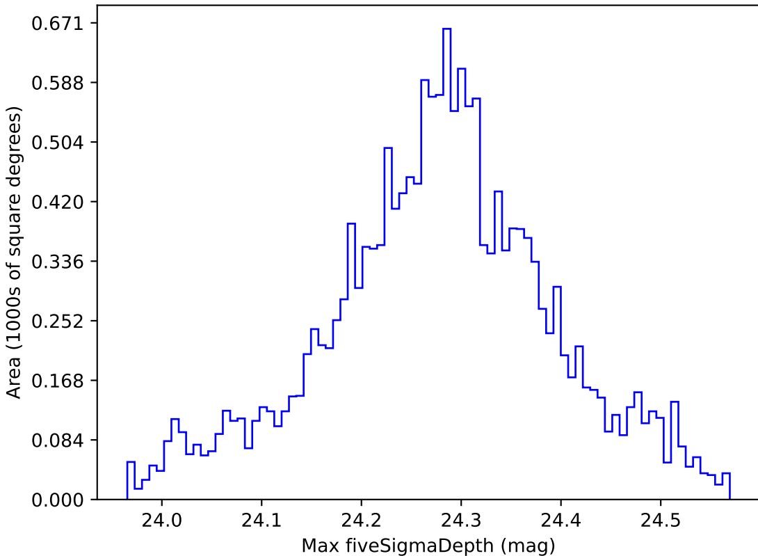
too_10_4v3.4_10yrs WFD i band: Max fiveSigmaDepth
