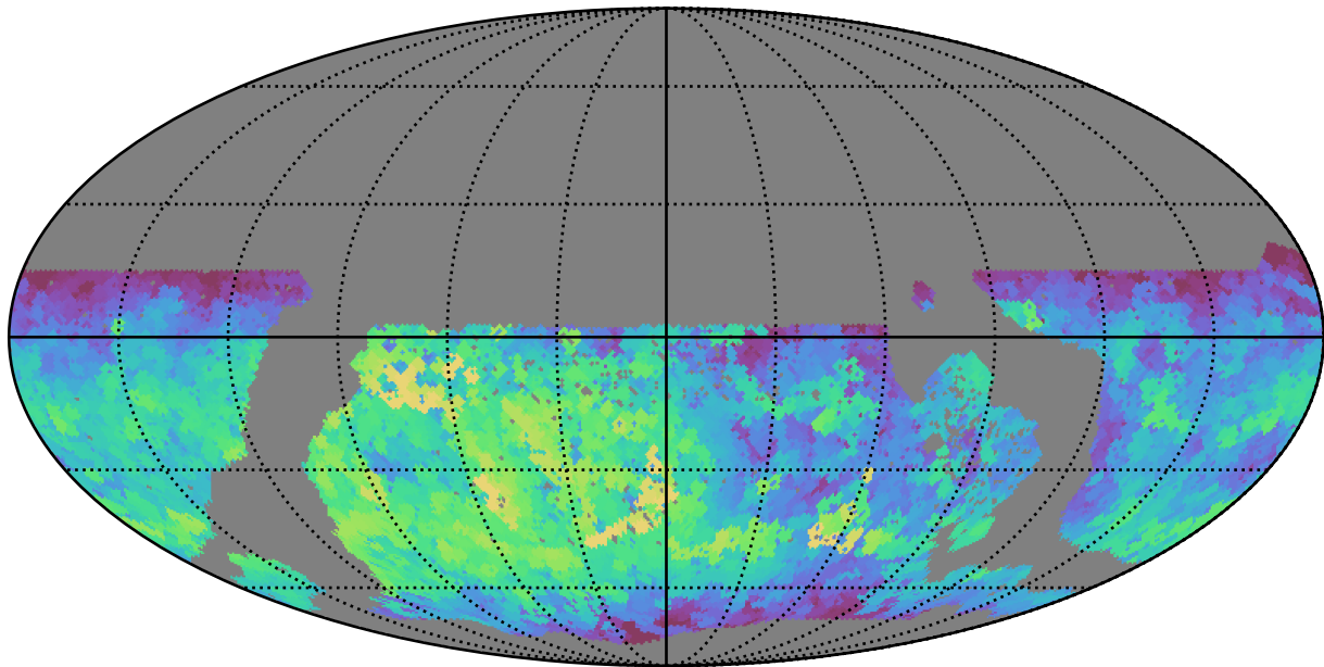
too_10_4v3.4_10yrs WFD g band: Max fiveSigmaDepth
