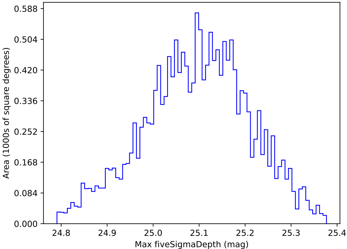
too_10_4v3.4_10yrs WFD g band: Max fiveSigmaDepth
