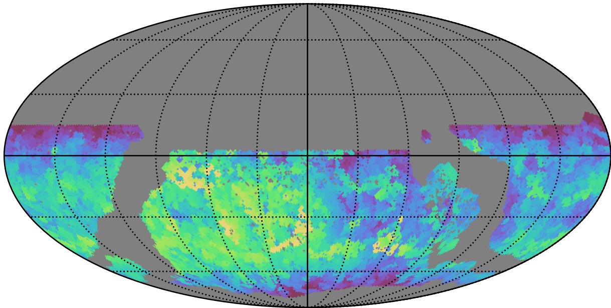
too_10_4v3.4_10yrs WFD all bands: Max fiveSigmaDepth
