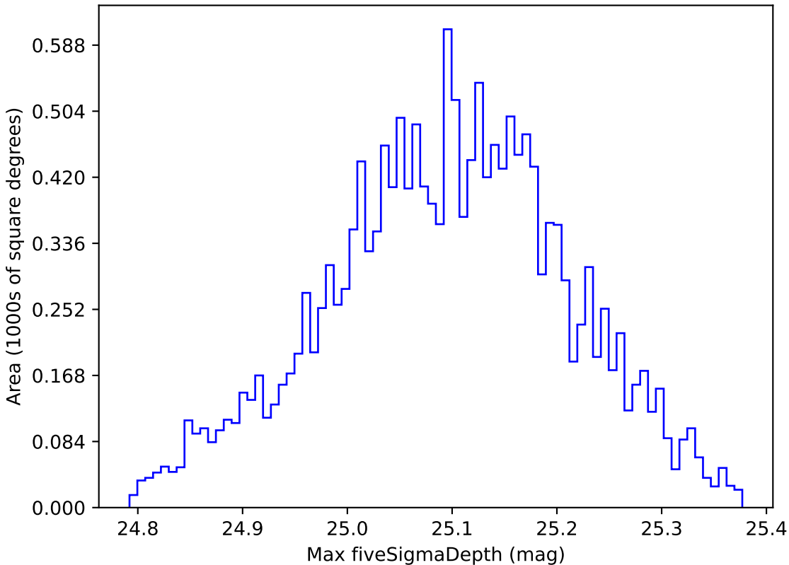
too_10_4v3.4_10yrs WFD all bands: Max fiveSigmaDepth
