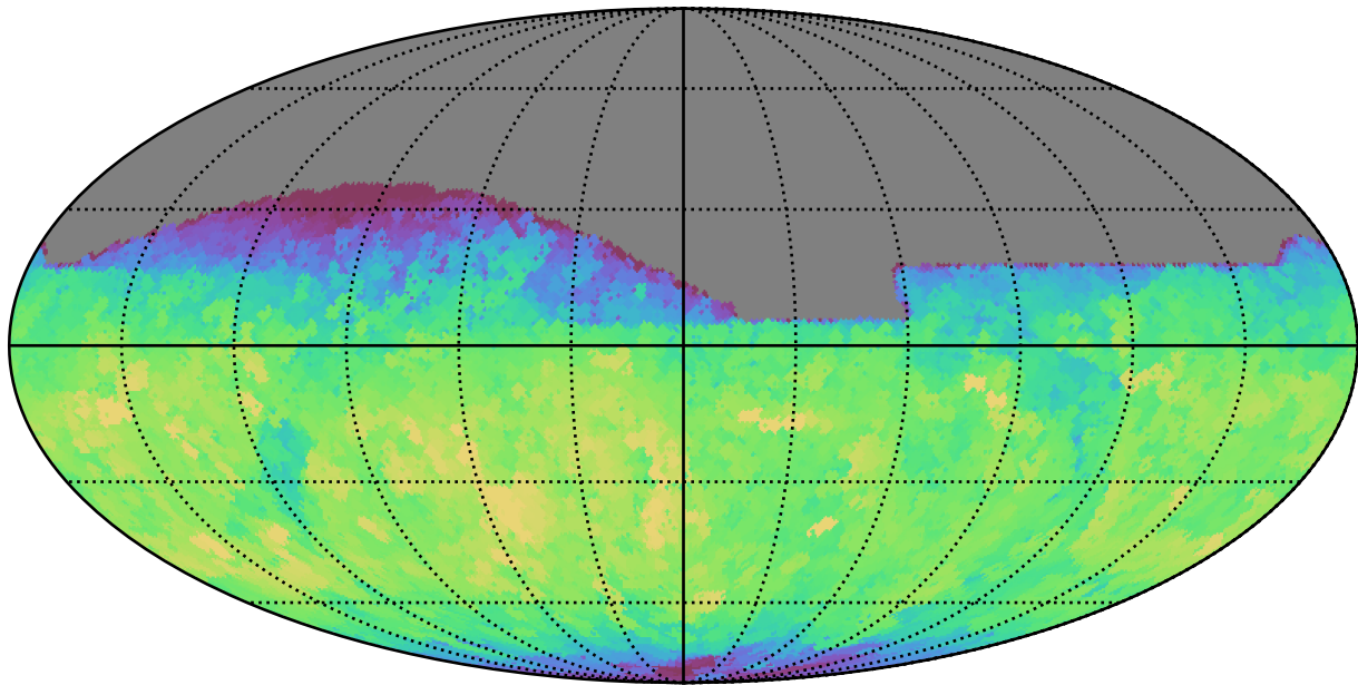
too_10_4v3.4_10yrs All sky z band: Max fiveSigmaDepth
