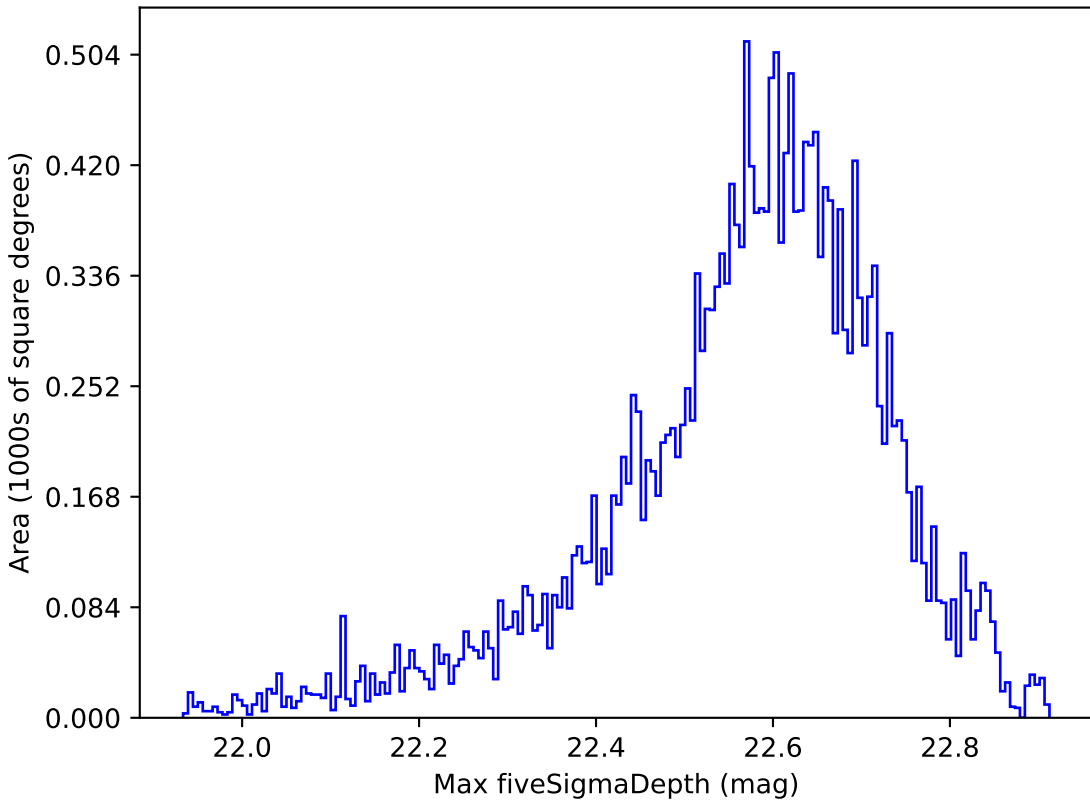
too_10_4v3.4_10yrs All sky y band: Max fiveSigmaDepth
