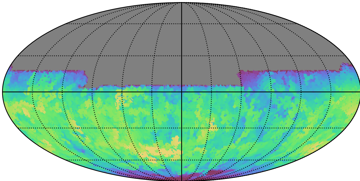
too_10_4v3.4_10yrs All sky u band: Max fiveSigmaDepth
