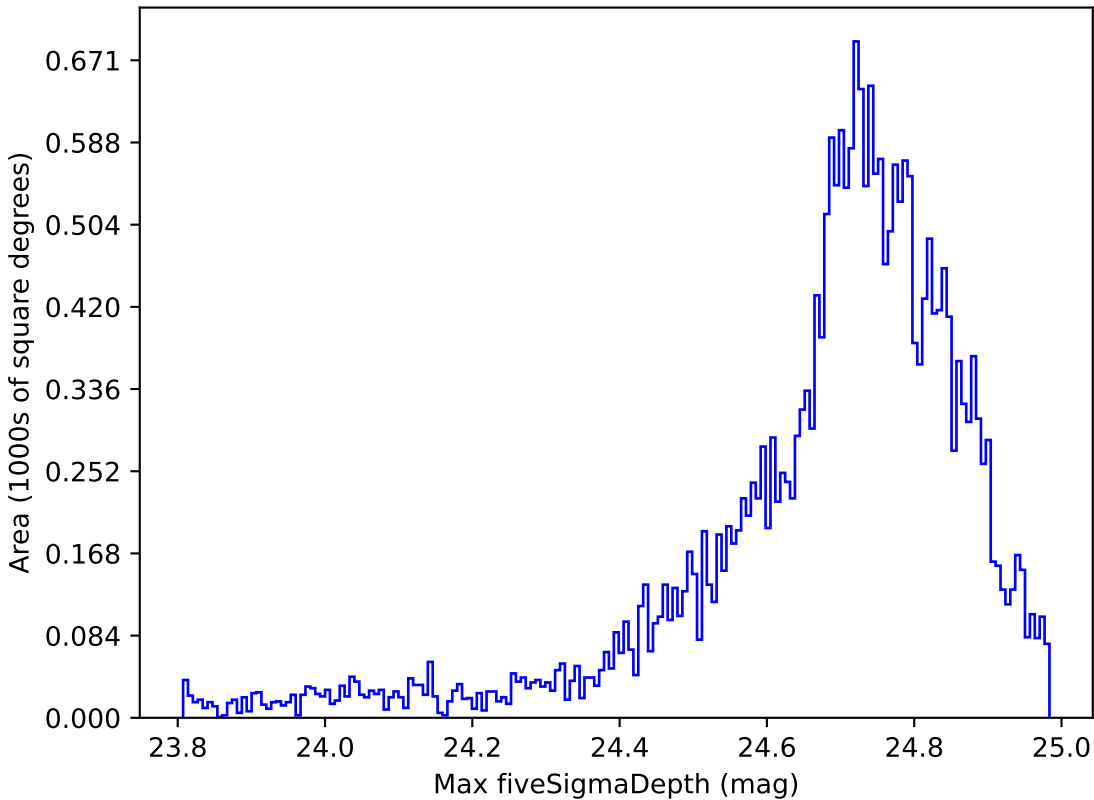
too_10_4v3.4_10yrs All sky r band: Max fiveSigmaDepth
