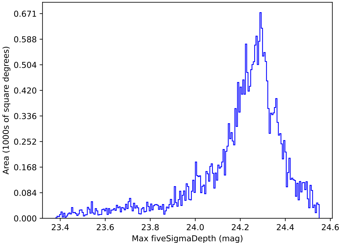
too_10_4v3.4_10yrs All sky i band: Max fiveSigmaDepth
