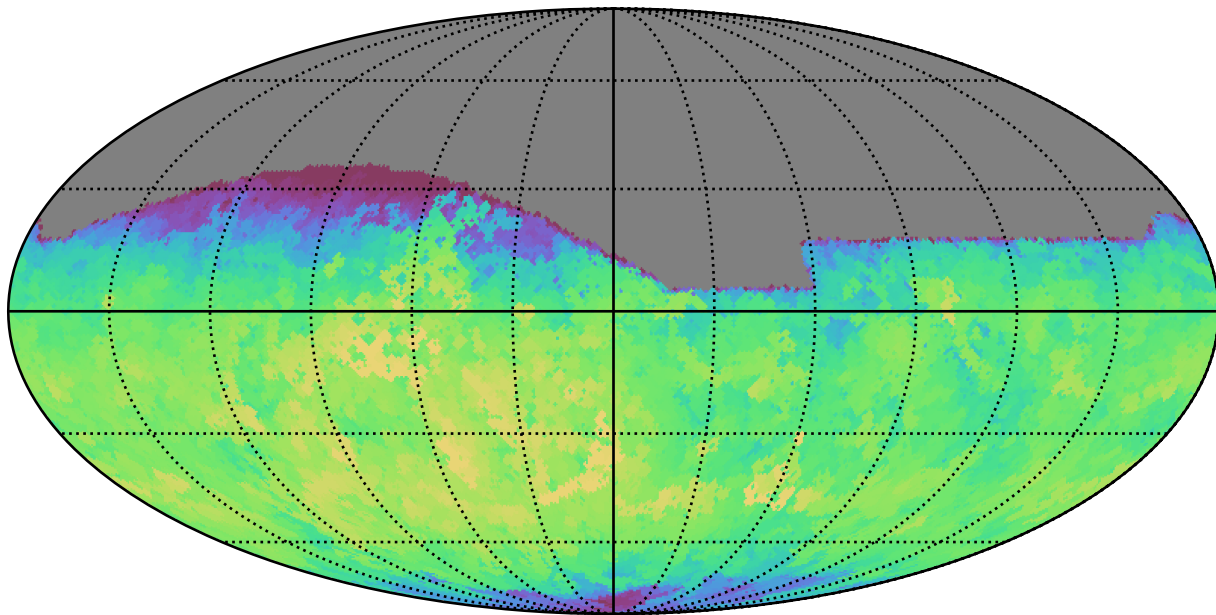
too_10_4v3.4_10yrs All sky g band: Max fiveSigmaDepth
