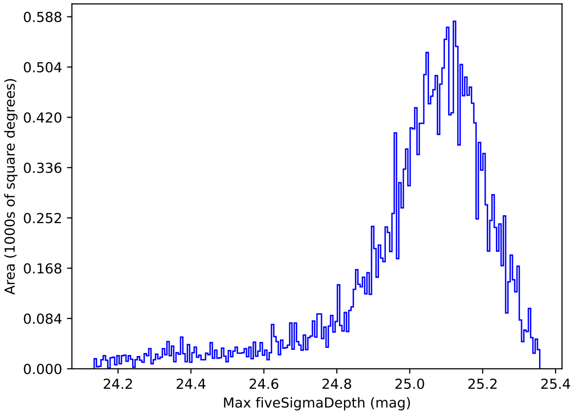
too_10_4v3.4_10yrs All sky g band: Max fiveSigmaDepth
