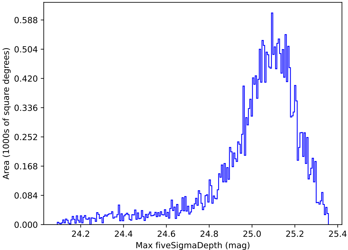
too_10_4v3.4_10yrs All sky all bands: Max fiveSigmaDepth
