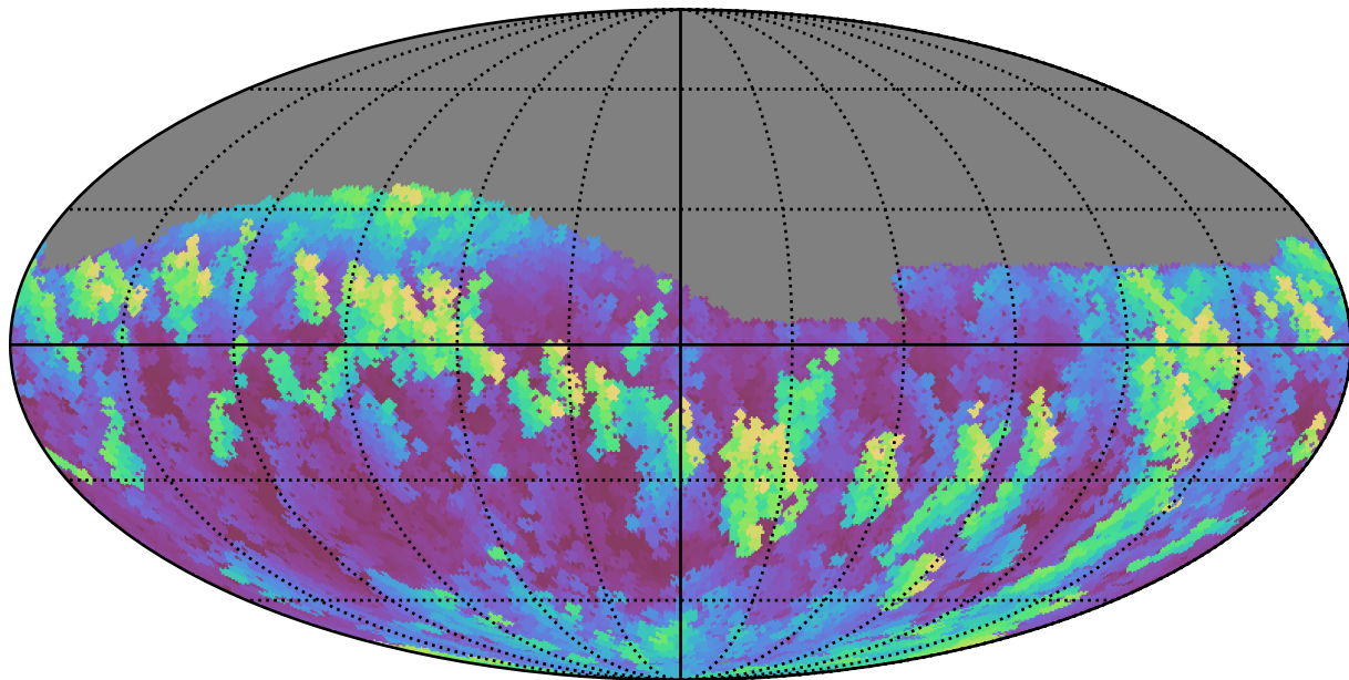
too_10_4v3.4_10yrs Yr 1 z band: Max airmass
