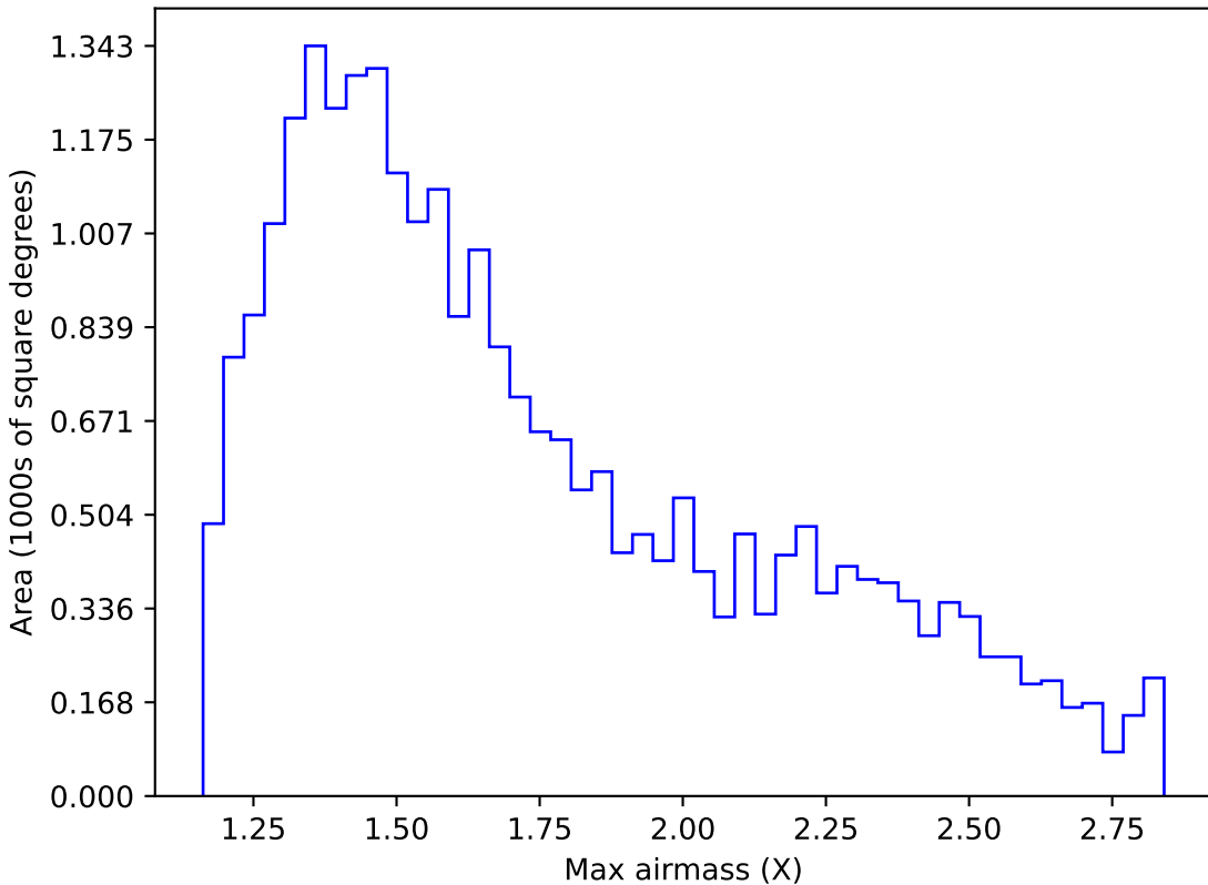
too_10_4v3.4_10yrs Yr 1 z band: Max airmass
