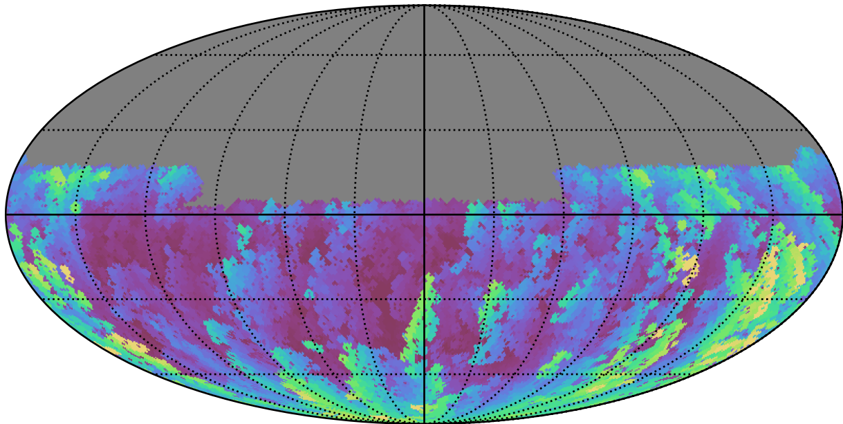
too_10_4v3.4_10yrs Yr 1 u band: Max airmass
