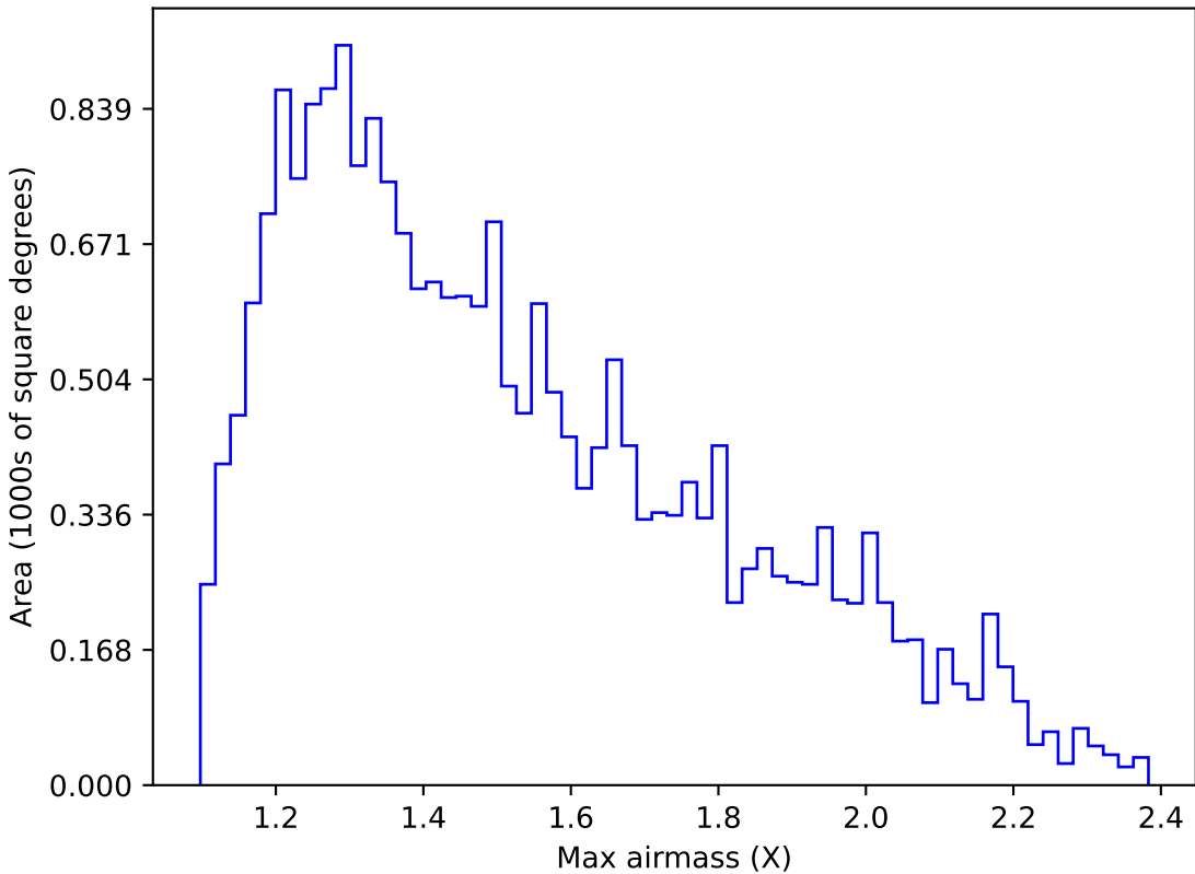
too_10_4v3.4_10yrs Yr 1 u band: Max airmass
