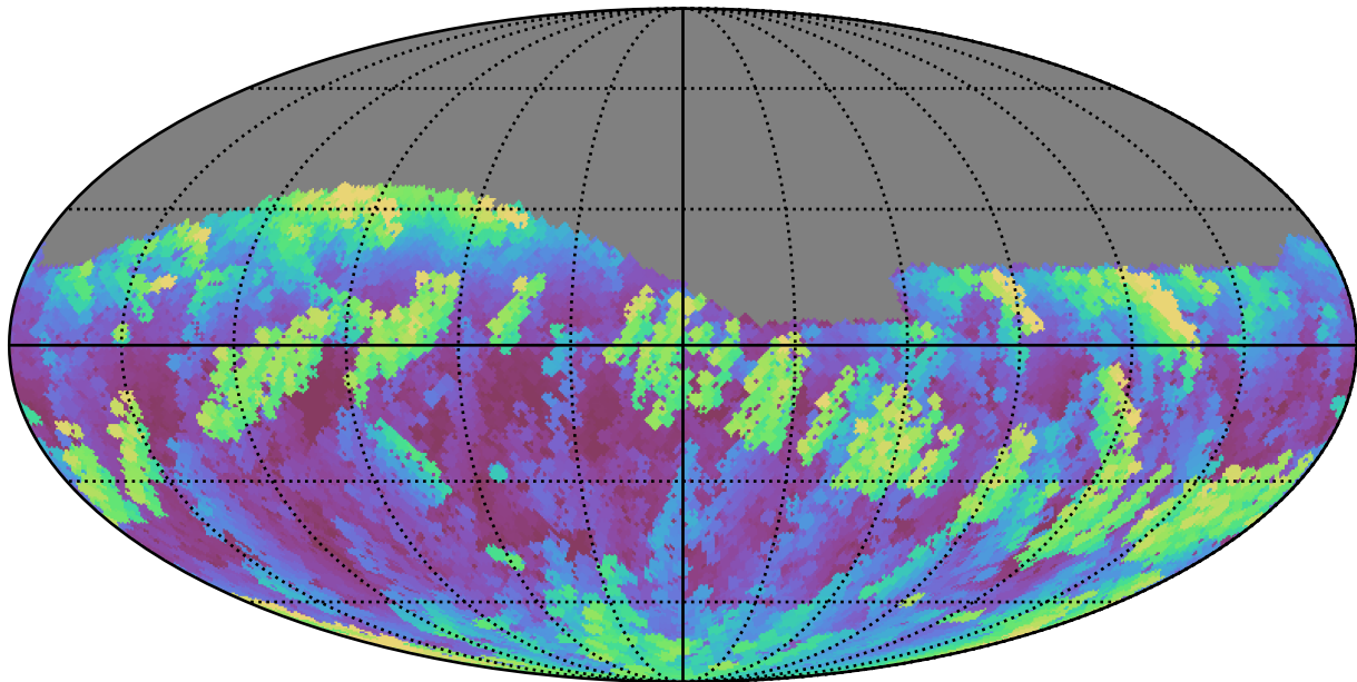
too_10_4v3.4_10yrs Yr 1 r band: Max airmass
