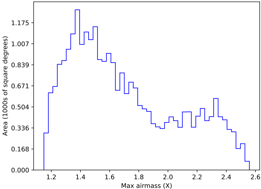
too_10_4v3.4_10yrs Yr 1 r band: Max airmass
