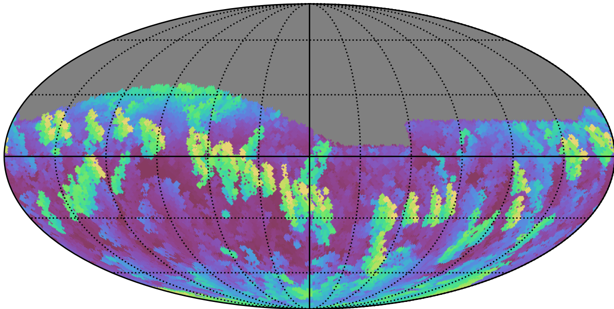
too_10_4v3.4_10yrs Yr 1 i band: Max airmass
