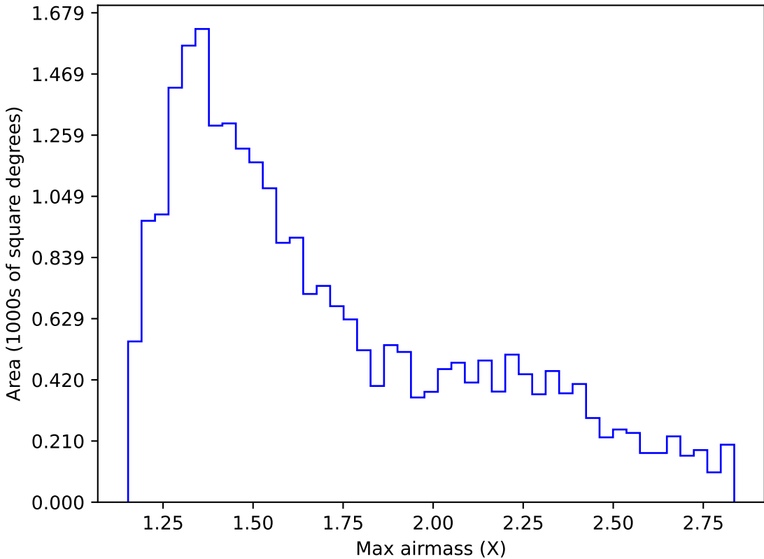
too_10_4v3.4_10yrs Yr 1 i band: Max airmass
