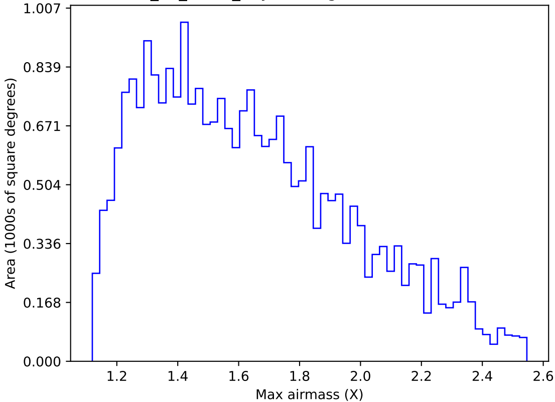
too_10_4v3.4_10yrs Yr 1 g band: Max airmass
