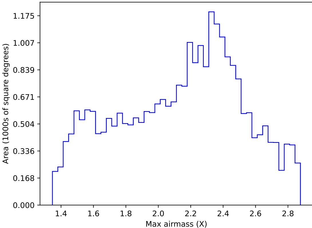
too_10_4v3.4_10yrs Yr 1 all bands: Max airmass
