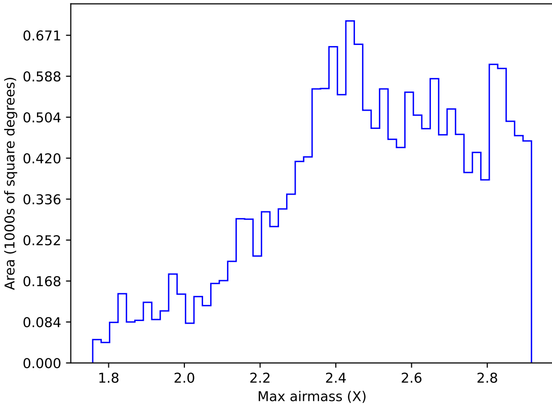
too_10_4v3.4_10yrs WFD z band: Max airmass
