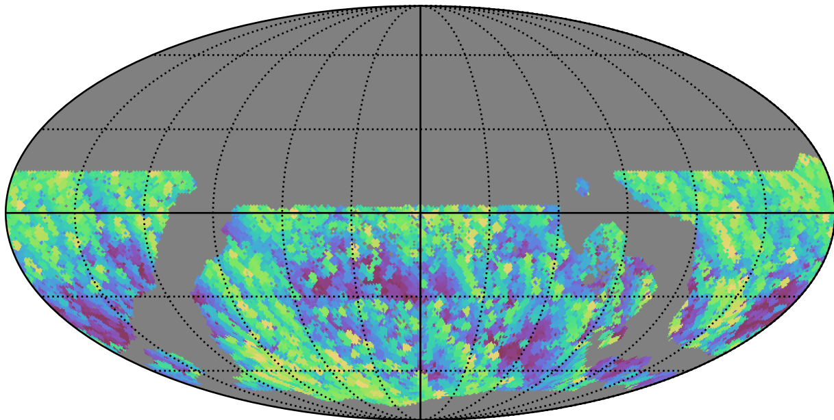
too_10_4v3.4_10yrs WFD y band: Max airmass
