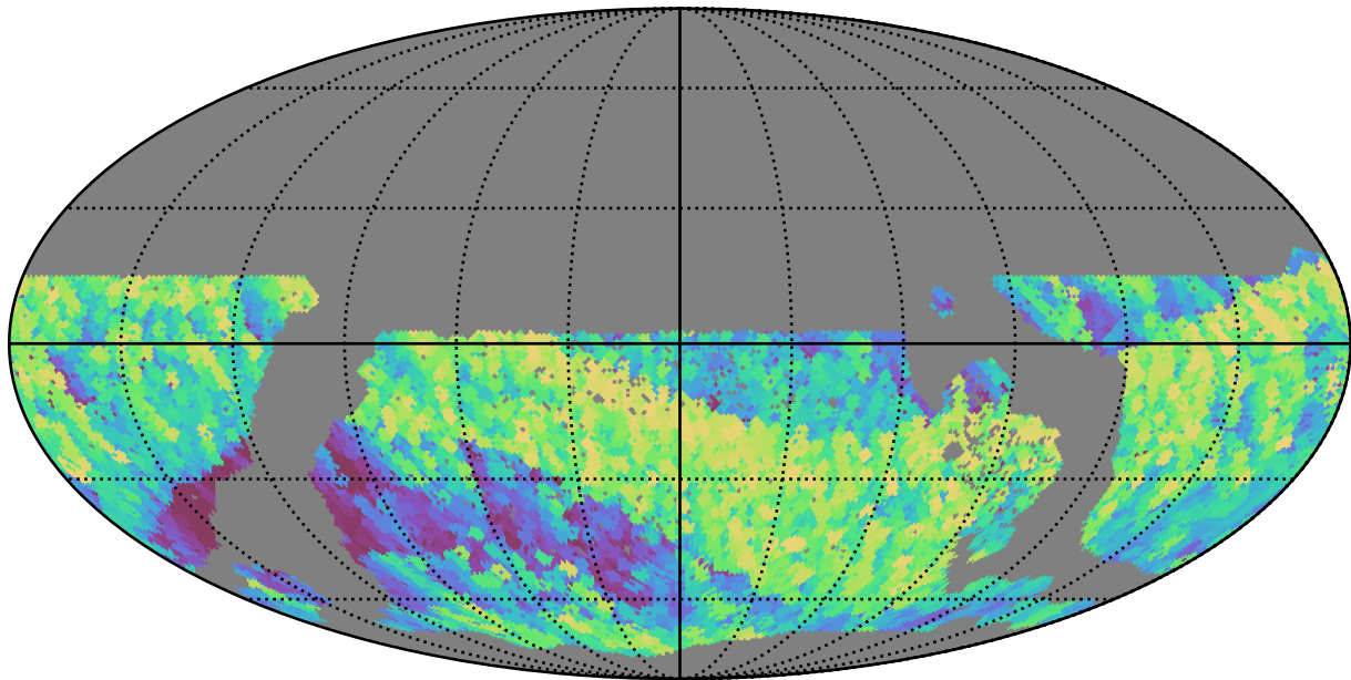
too_10_4v3.4_10yrs WFD i band: Max airmass
