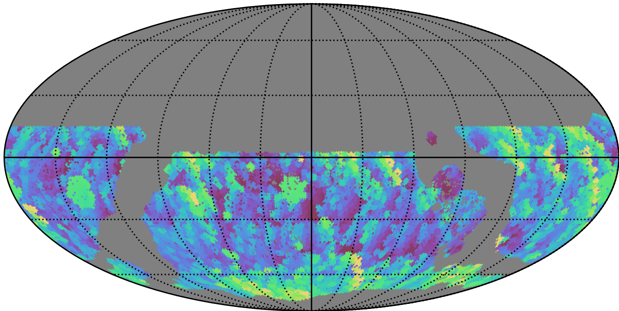
too_10_4v3.4_10yrs WFD g band: Max airmass
