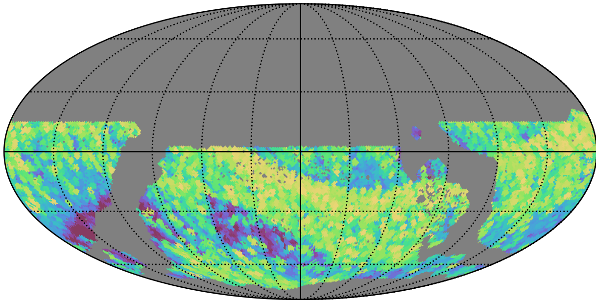
too_10_4v3.4_10yrs WFD all bands: Max airmass
