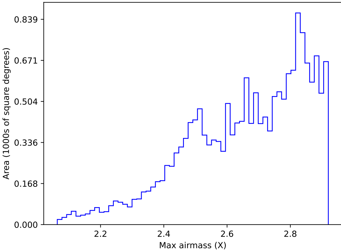
too_10_4v3.4_10yrs WFD all bands: Max airmass
