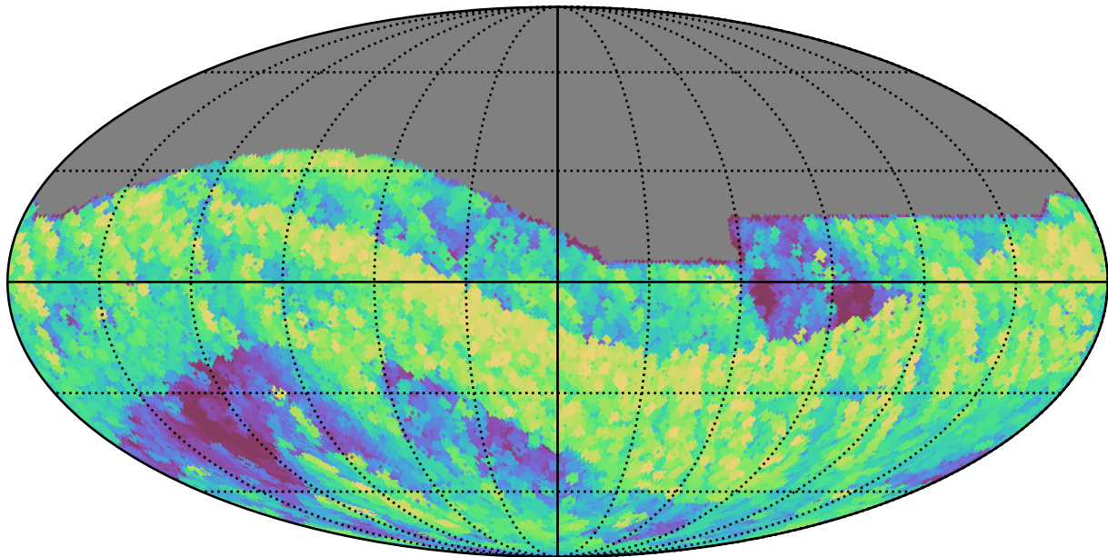
too_10_4v3.4_10yrs All sky z band: Max airmass
