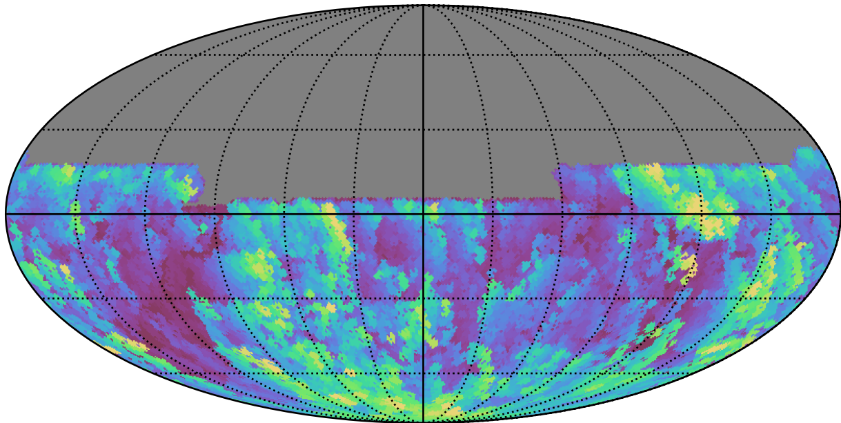
too_10_4v3.4_10yrs All sky u band: Max airmass
