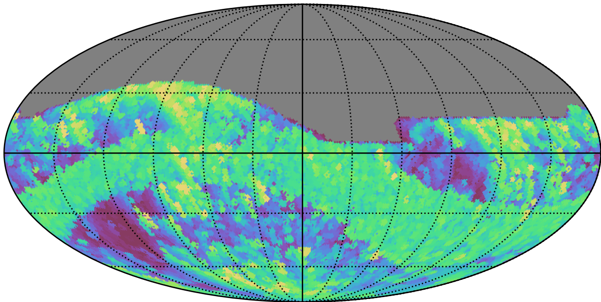
too_10_4v3.4_10yrs All sky r band: Max airmass
