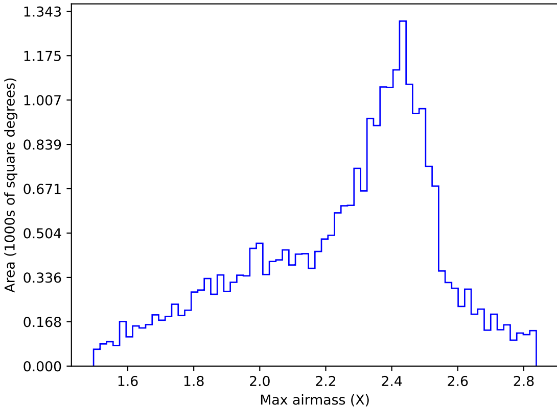
too_10_4v3.4_10yrs All sky r band: Max airmass
