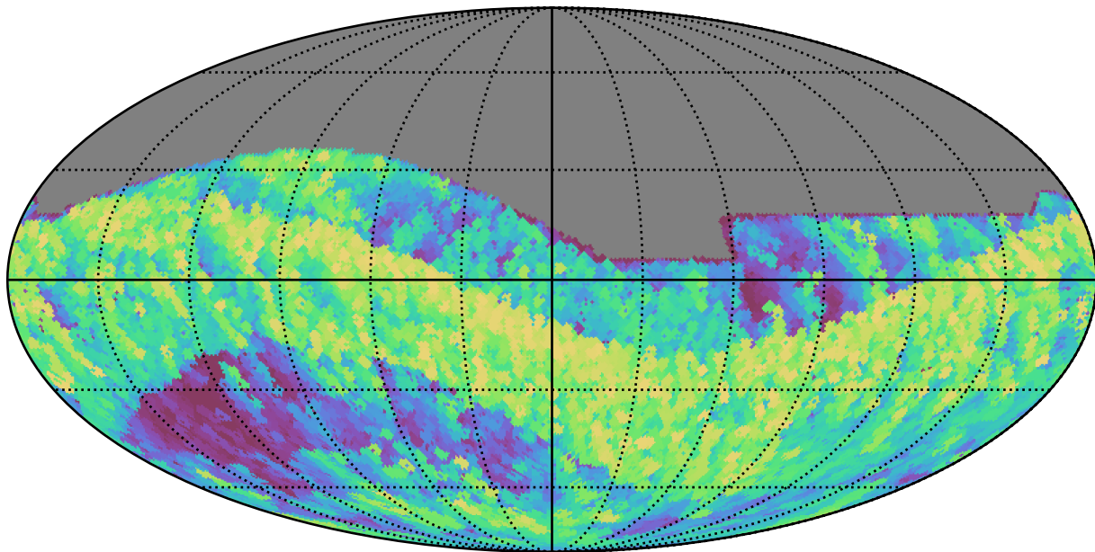
too_10_4v3.4_10yrs All sky i band: Max airmass
