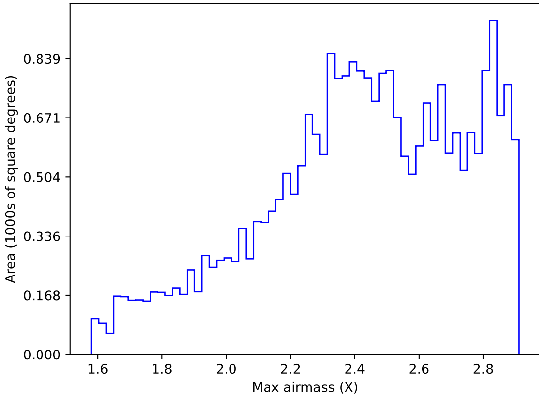
too_10_4v3.4_10yrs All sky i band: Max airmass
