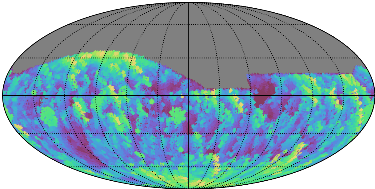
too_10_4v3.4_10yrs All sky g band: Max airmass
