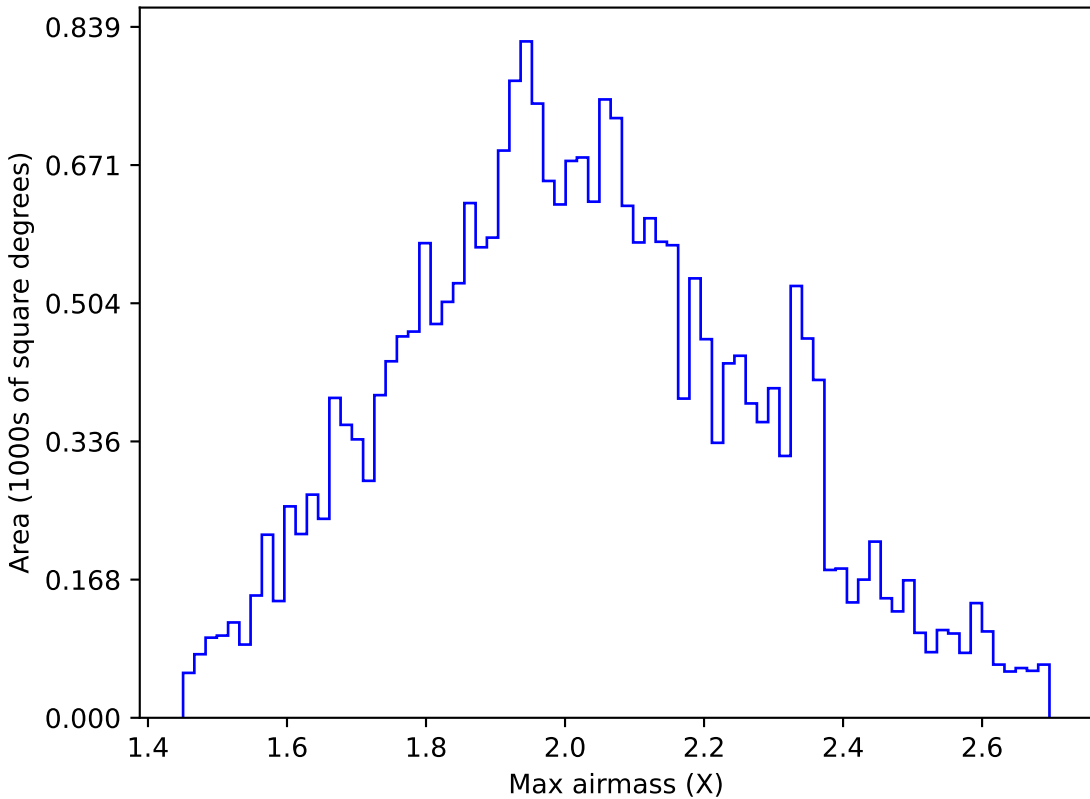
too_10_4v3.4_10yrs All sky g band: Max airmass
