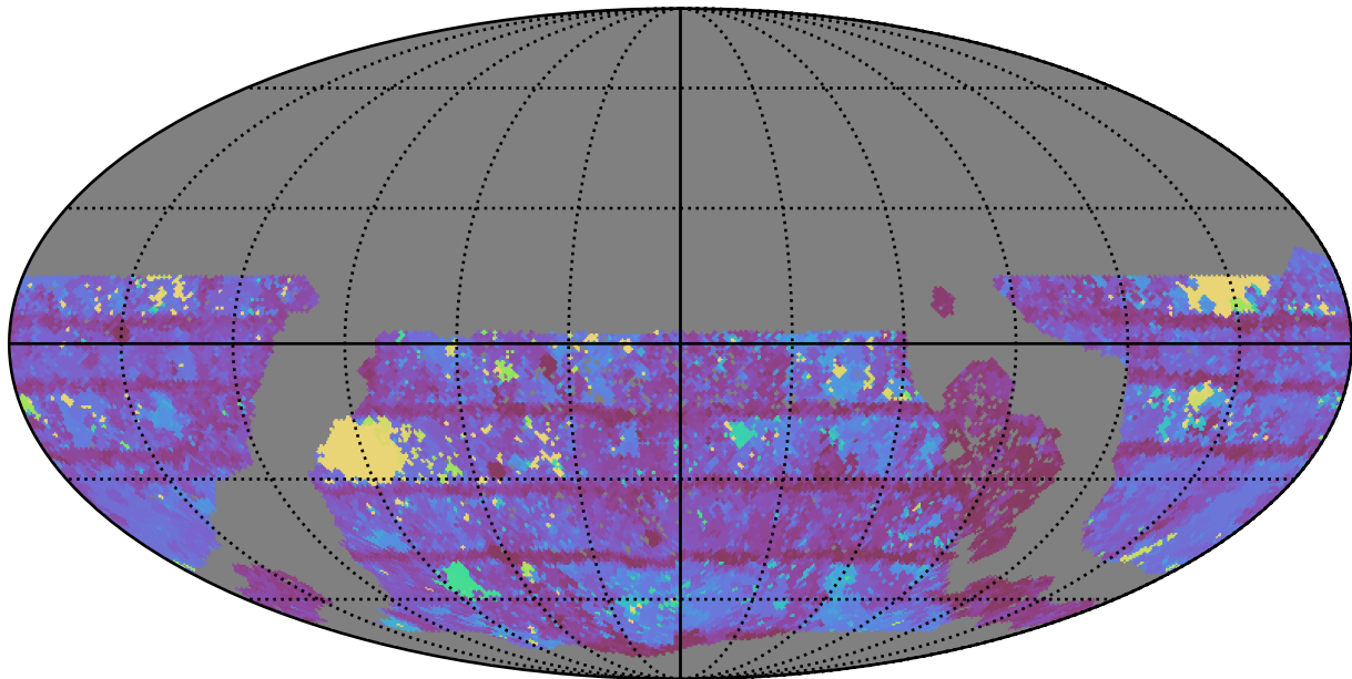
too_10_4v3.4_10yrs WFD z band: Max Inter-Night Gap
