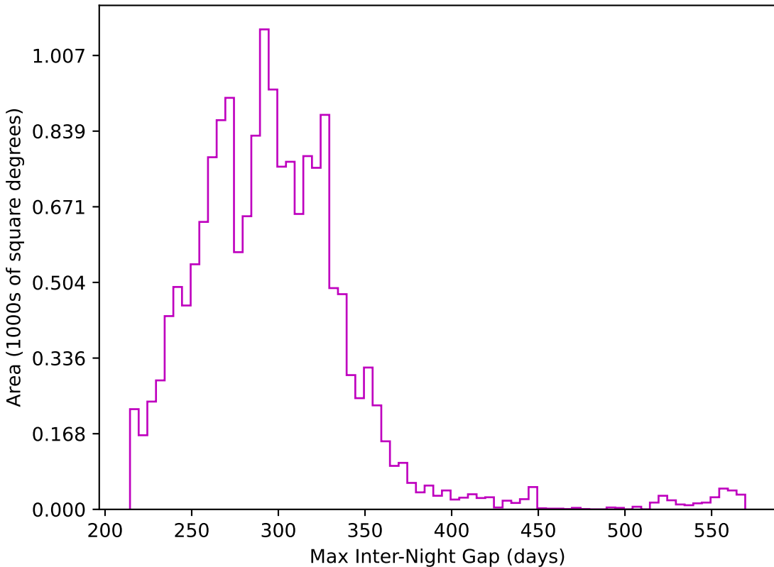
too_10_4v3.4_10yrs WFD z band: Max Inter-Night Gap
