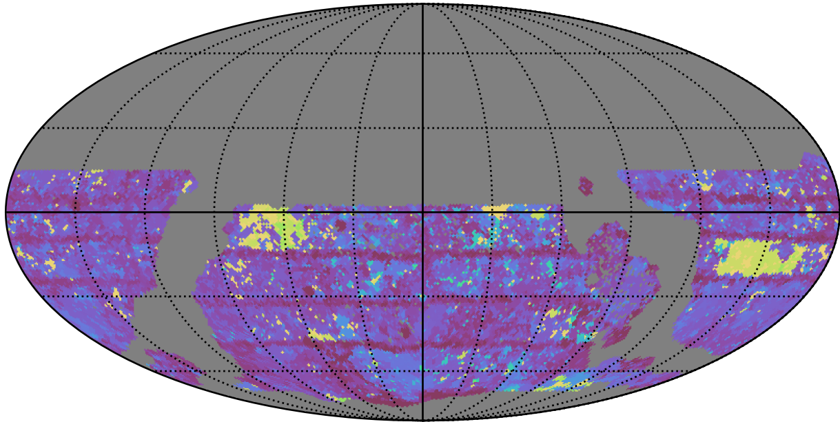
too_10_4v3.4_10yrs WFD y band: Max Inter-Night Gap
