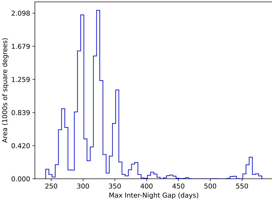
too_10_4v3.4_10yrs WFD y band: Max Inter-Night Gap
