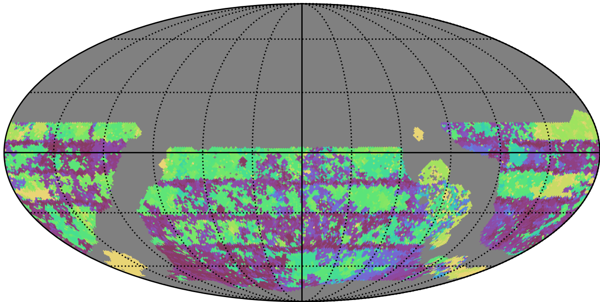
too_10_4v3.4_10yrs WFD u band: Max Inter-Night Gap
