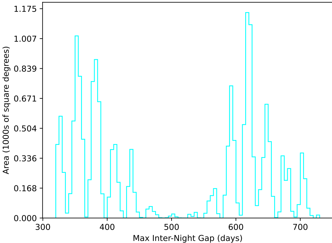
too_10_4v3.4_10yrs WFD u band: Max Inter-Night Gap
