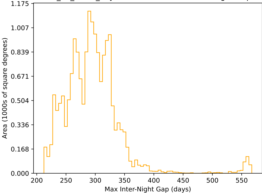
too_10_4v3.4_10yrs WFD r band: Max Inter-Night Gap
