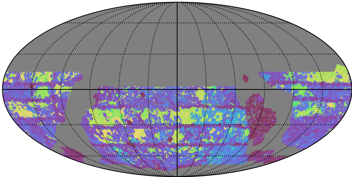
too_10_4v3.4_10yrs WFD g band: Max Inter-Night Gap
