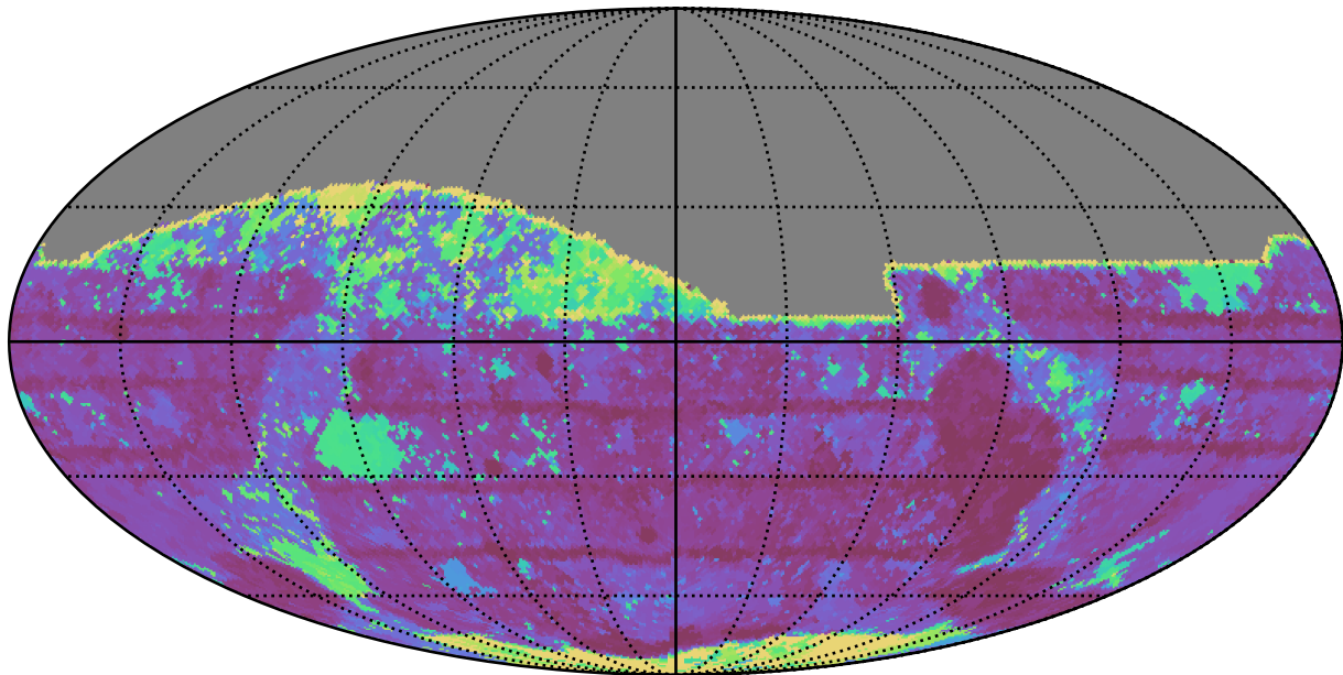
too_10_4v3.4_10yrs All sky z band: Max Inter-Night Gap
