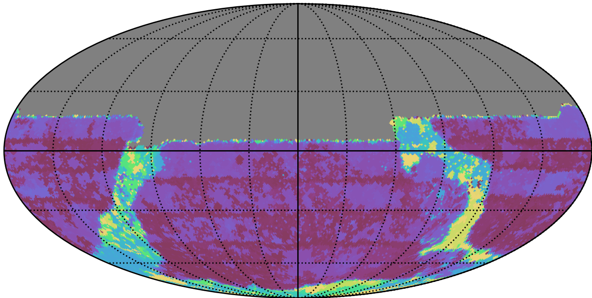
too_10_4v3.4_10yrs All sky u band: Max Inter-Night Gap
