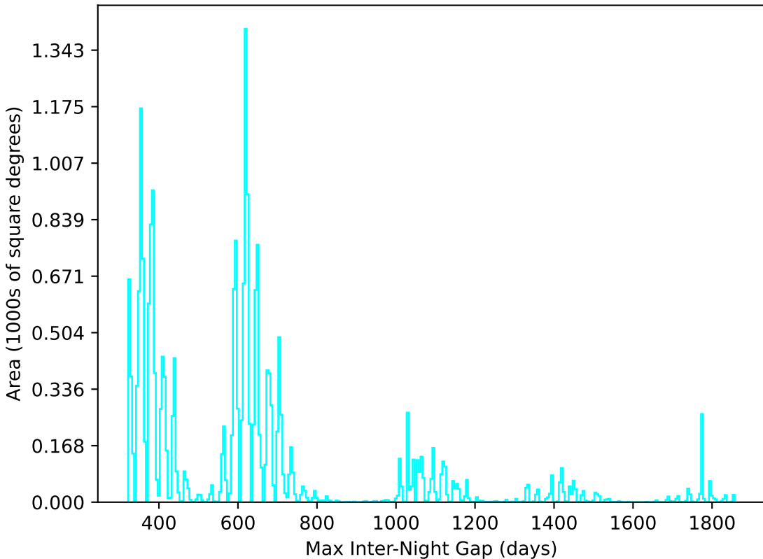
too_10_4v3.4_10yrs All sky u band: Max Inter-Night Gap
